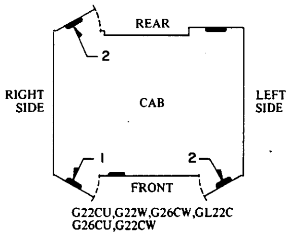
Cab Access Door Location Chart
