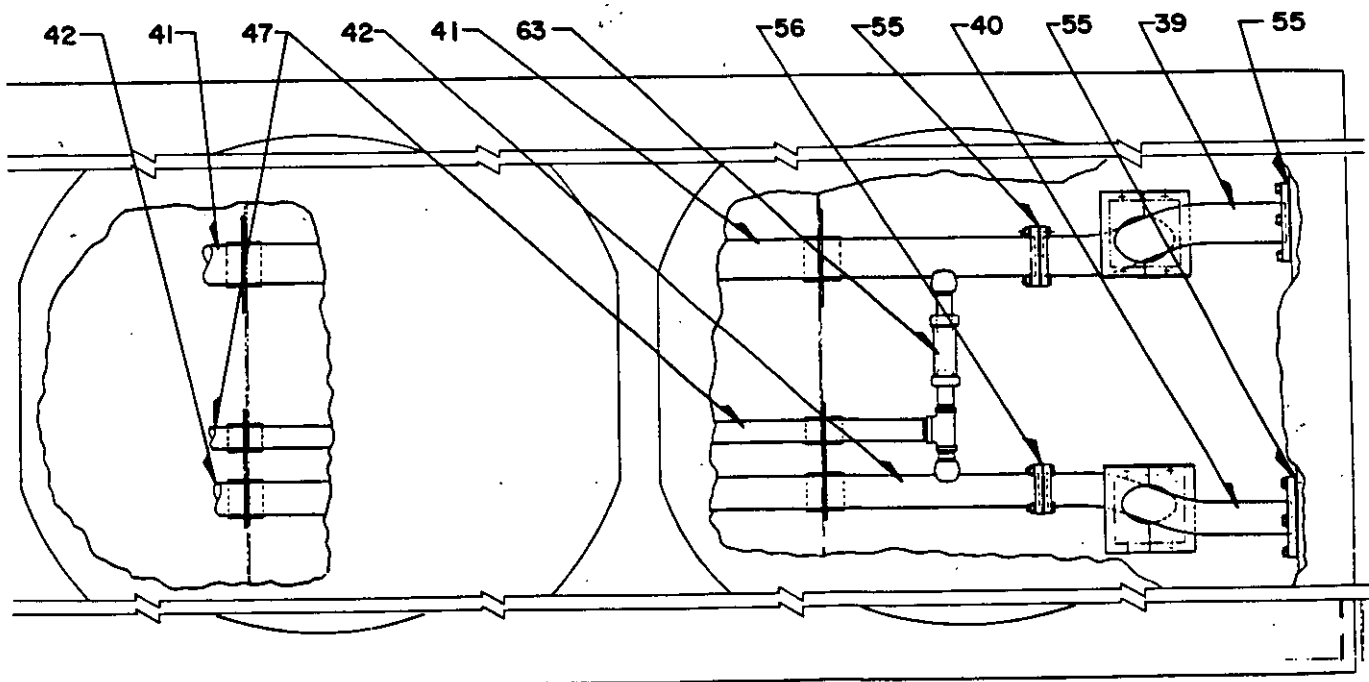
VIEW E-E TOP VIEW PLATE A513-E-12
