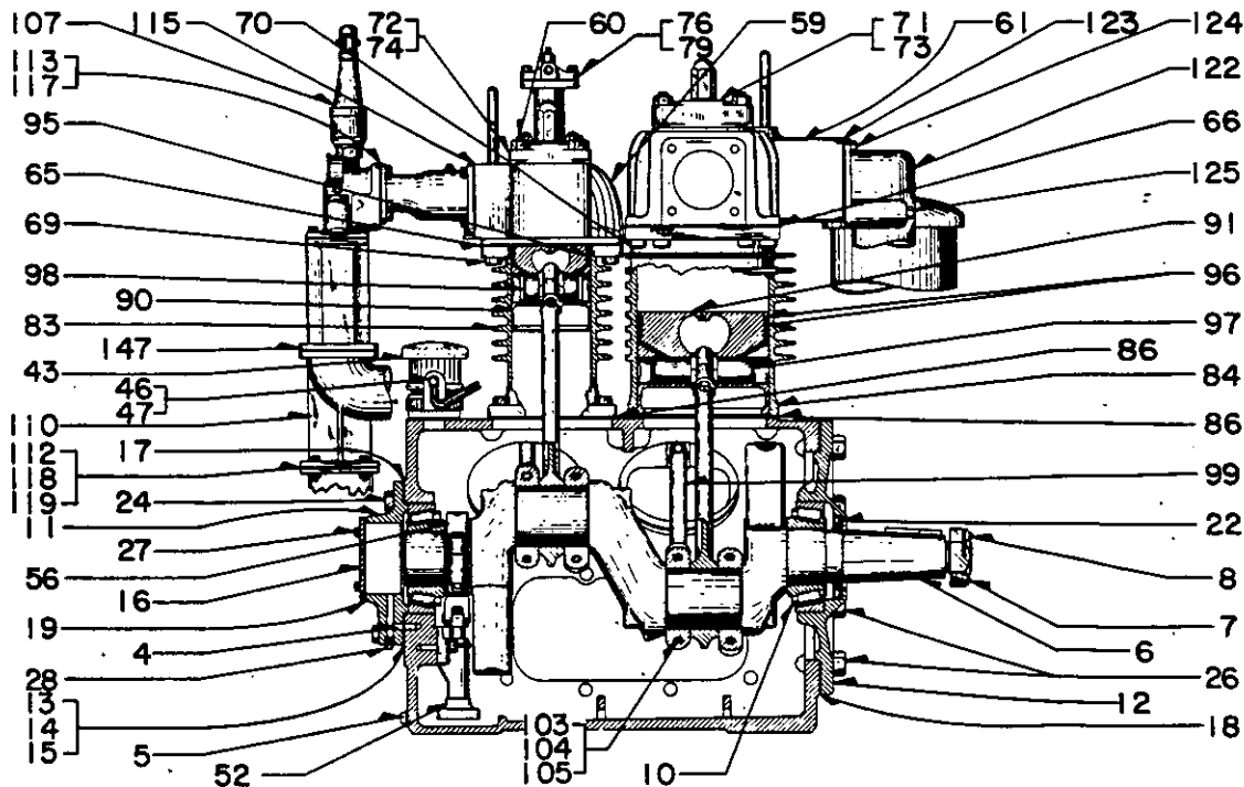
Side View Ref. No. 1 PLATE C1100-E-1
