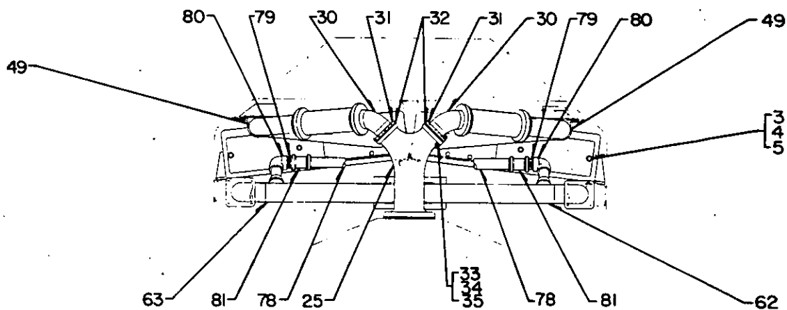
FRONT VIEW STARTING NOVEMBER, 1973 PLATE B543-E-6
