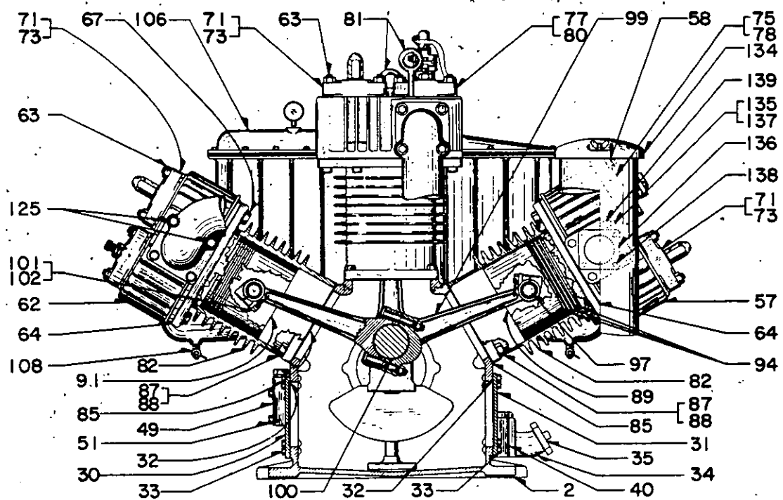
FRONT VIEW PLATE C1100-E-2
