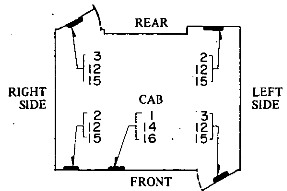
Locomotives With (5) Air Motors
